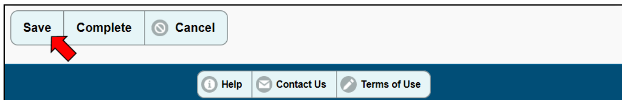
Figure 5: Save Progress
